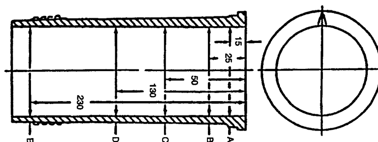
NOTE 1—Measurements are in millimetres. FIG. A1.5 Measurements of Cylinder Liner
