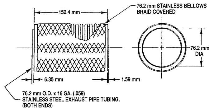
FIG. A3.2 Exhaust Barrel Diagram
