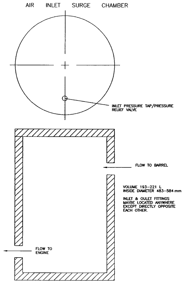
FIG. A2.2 Air Inlet Surge Chamber
