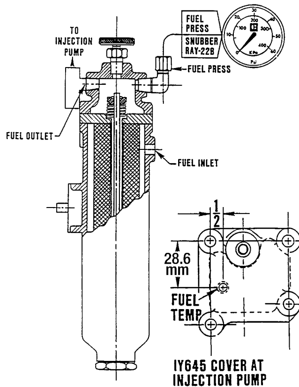
FIG. A6.1 Fuel Pressure and Temperature Measurement Locations
