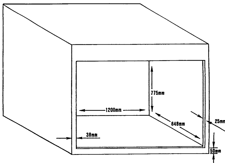
FIG. A11.4 Rating Booth
