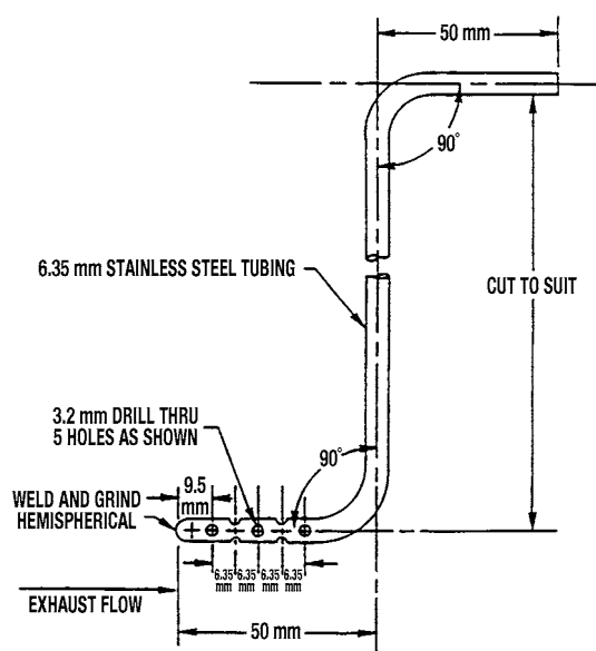
FIG. A3.5 Exhaust Gas Sample Probe
