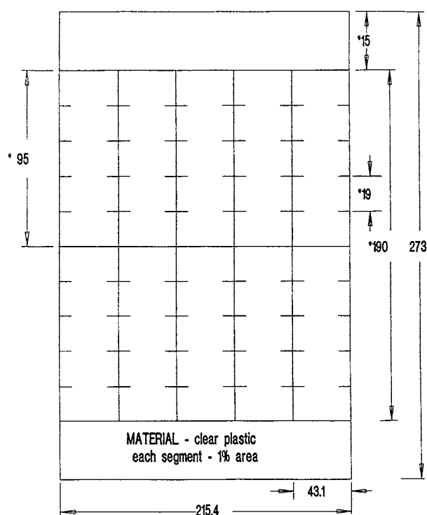
FIG. A11.3 Bore Polishing Grid
