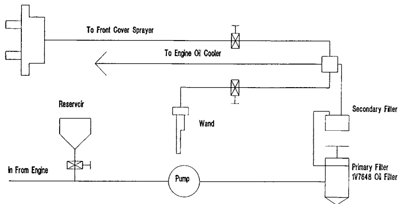
FIG. A9.4 Flushing Cart Flow Schematic
