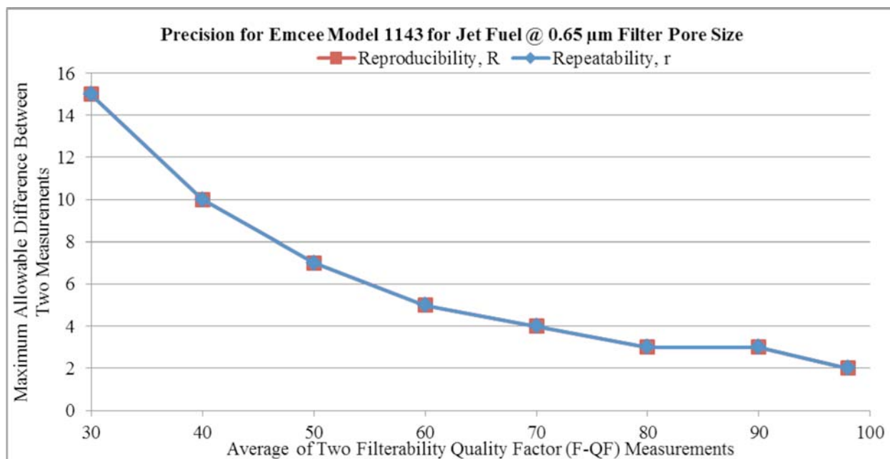
FIG. 4 Precision for Jet Fuel at 0.65 µm Filter Pore Size (Repeatability (r) and Reproducibility (R))
