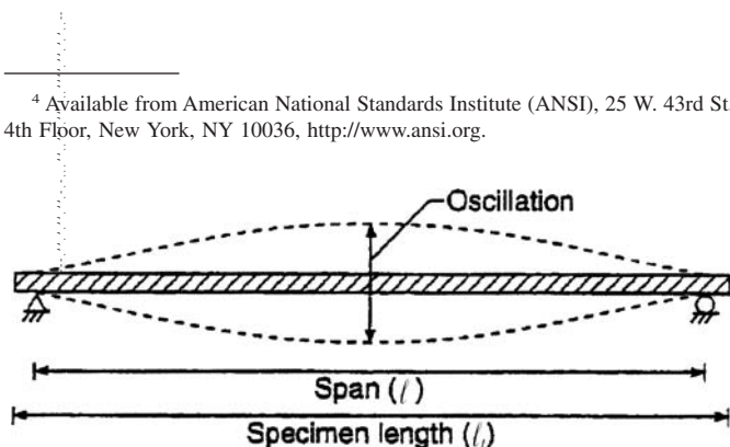
FIG. 1 Transverse Vibration in the Fundamental Mode
