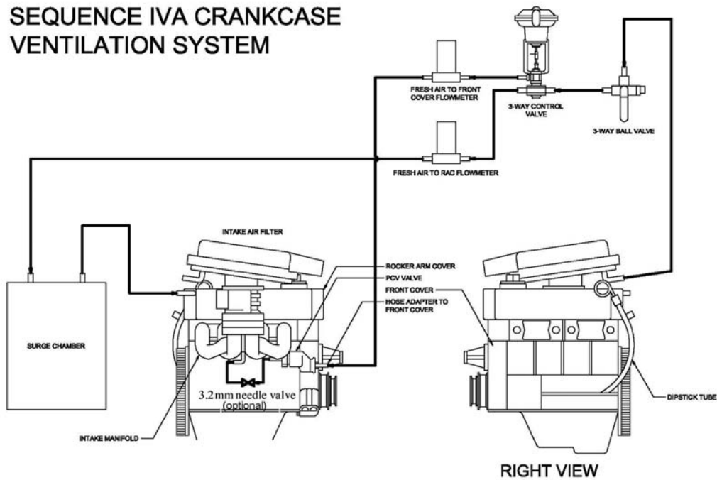
FIG. 3 Typical Crankcase Ventilation
