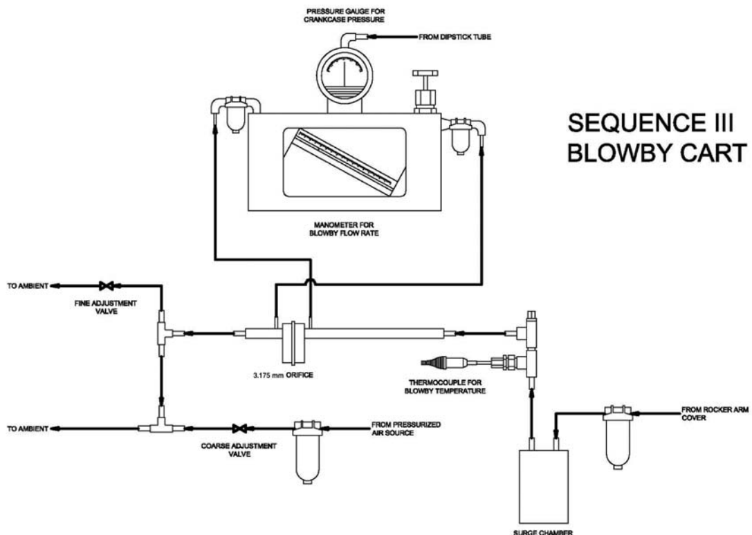
FIG. A3.18 Typical Alternate Measurement Device
