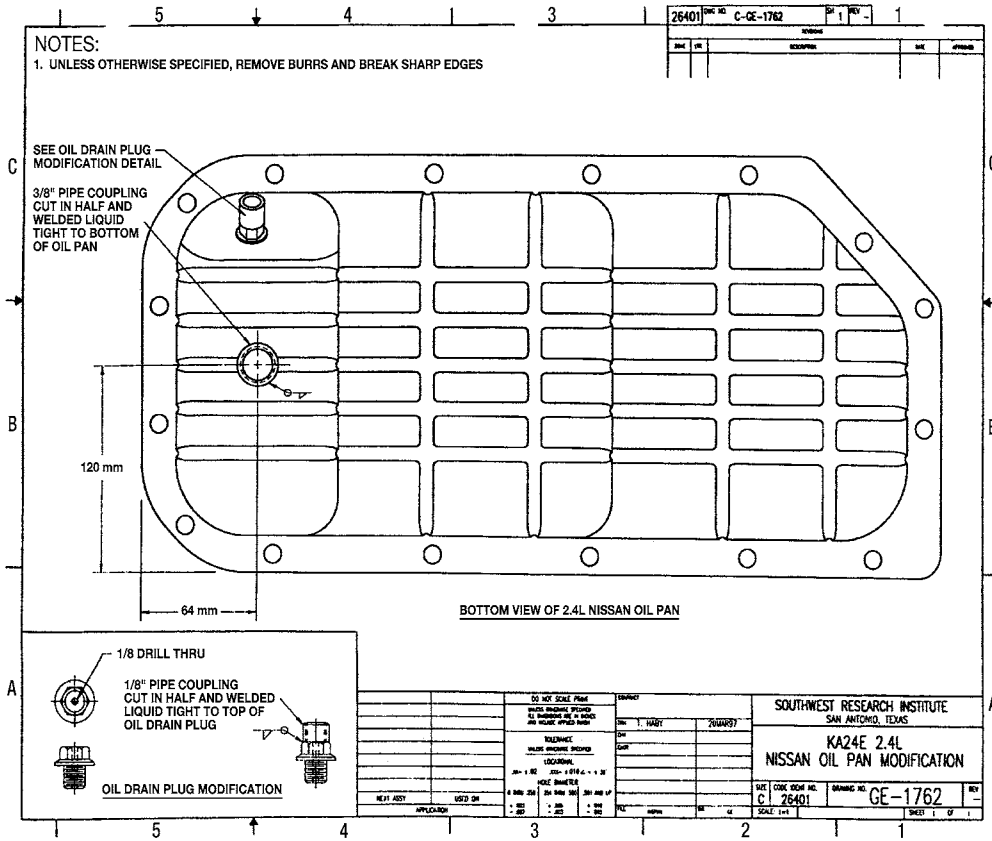
FIG. A3.6 Oil Pan Modification
