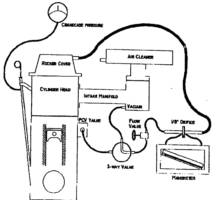
FIG. A3.17 Blow-by Measurement Equipment Schematic
