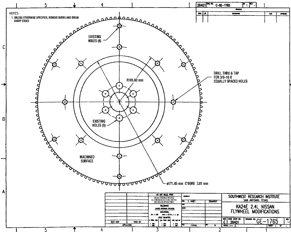
FIG. A3.13 Flywheel Modifications
