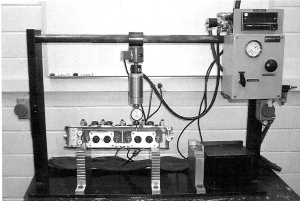
FIG. 10 Head Calibration
