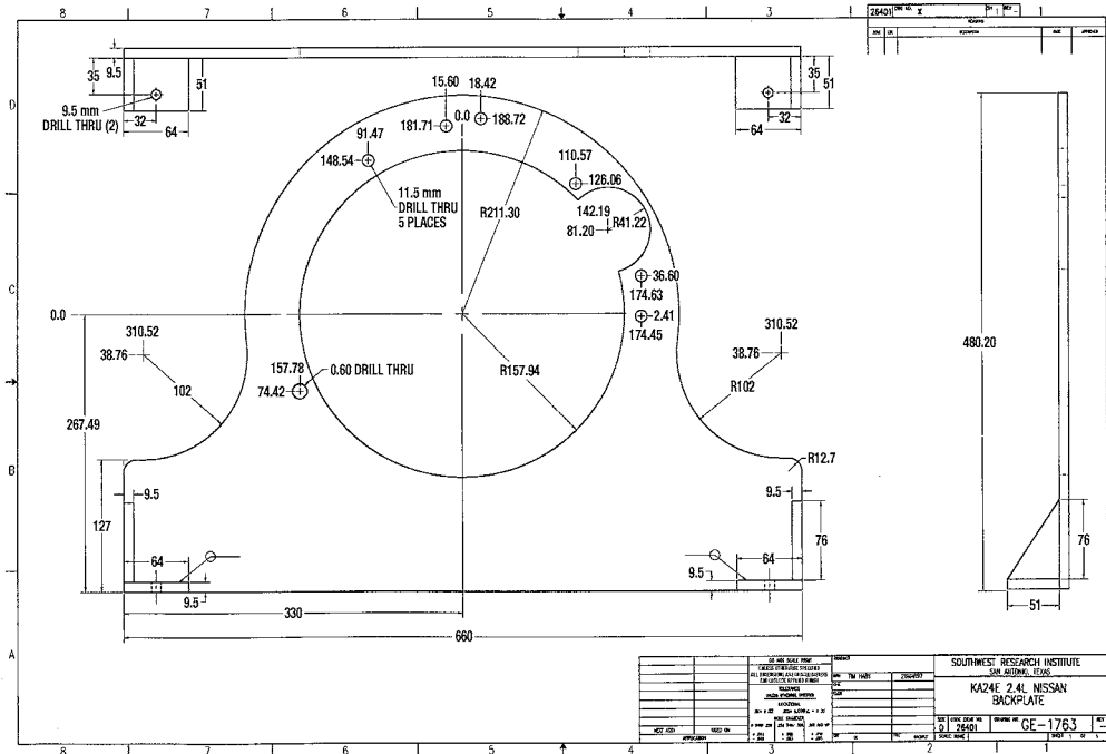
FIG. A3.12 Engine Backplate
