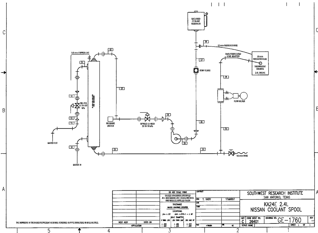
FIG. A3.7 Coolant Spool
