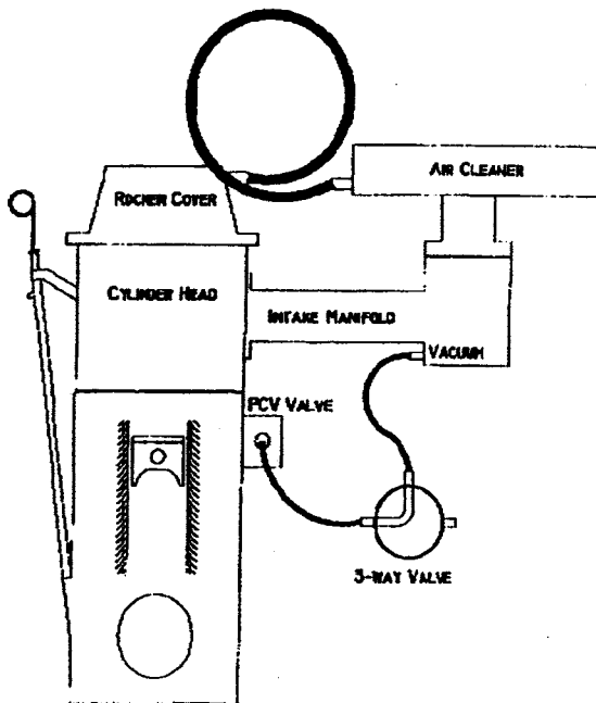
FIG. A3.17 Blow-by Measurement Equipment Schematic
