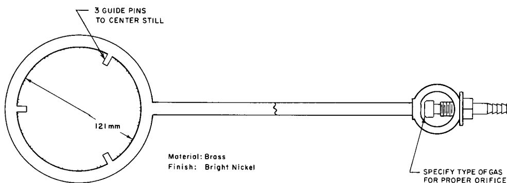
FIG. 2 Ring Burner with 125-mm Inside Diameter
