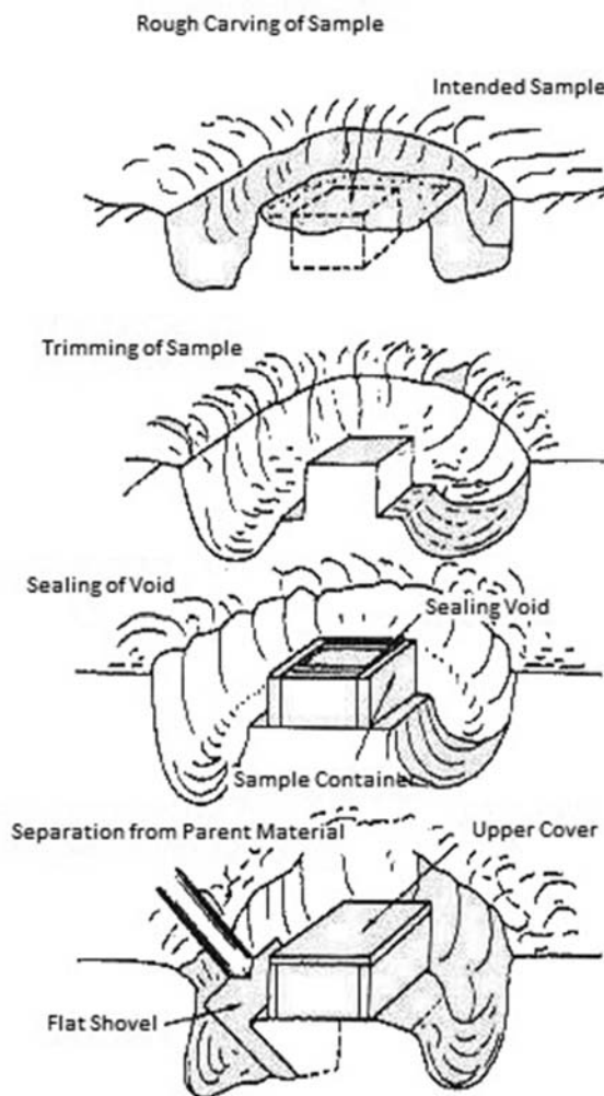
FIG. 1 Procedure for Rectangular Block Sampling
