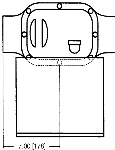
FIG. A1.4 Temperature Probe Location
