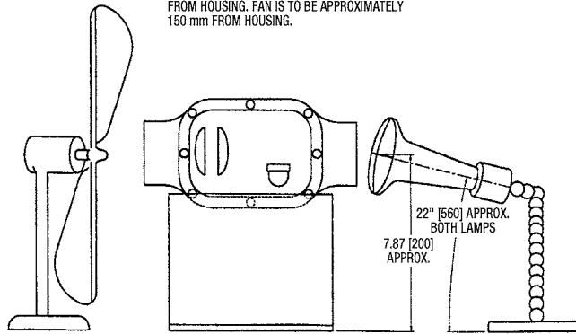
NOTE 1—Dimensions are in inches (millimetres). FIG. A1.3 Heat Lamp And Fan Arrangement
