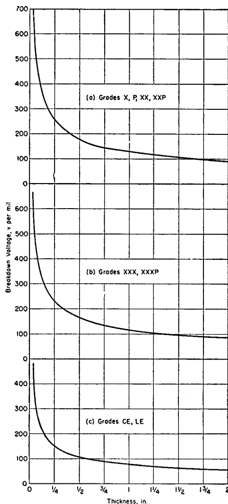
FIG. X3.1 Typical Dielectric Strength Values
