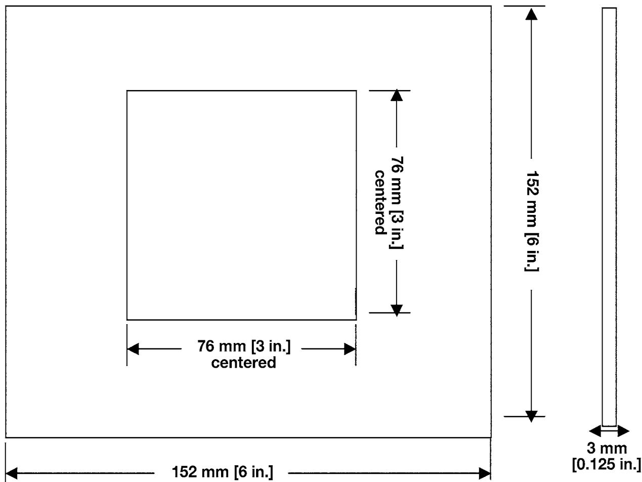
FIG. 3 Specimen Mounting Plate
