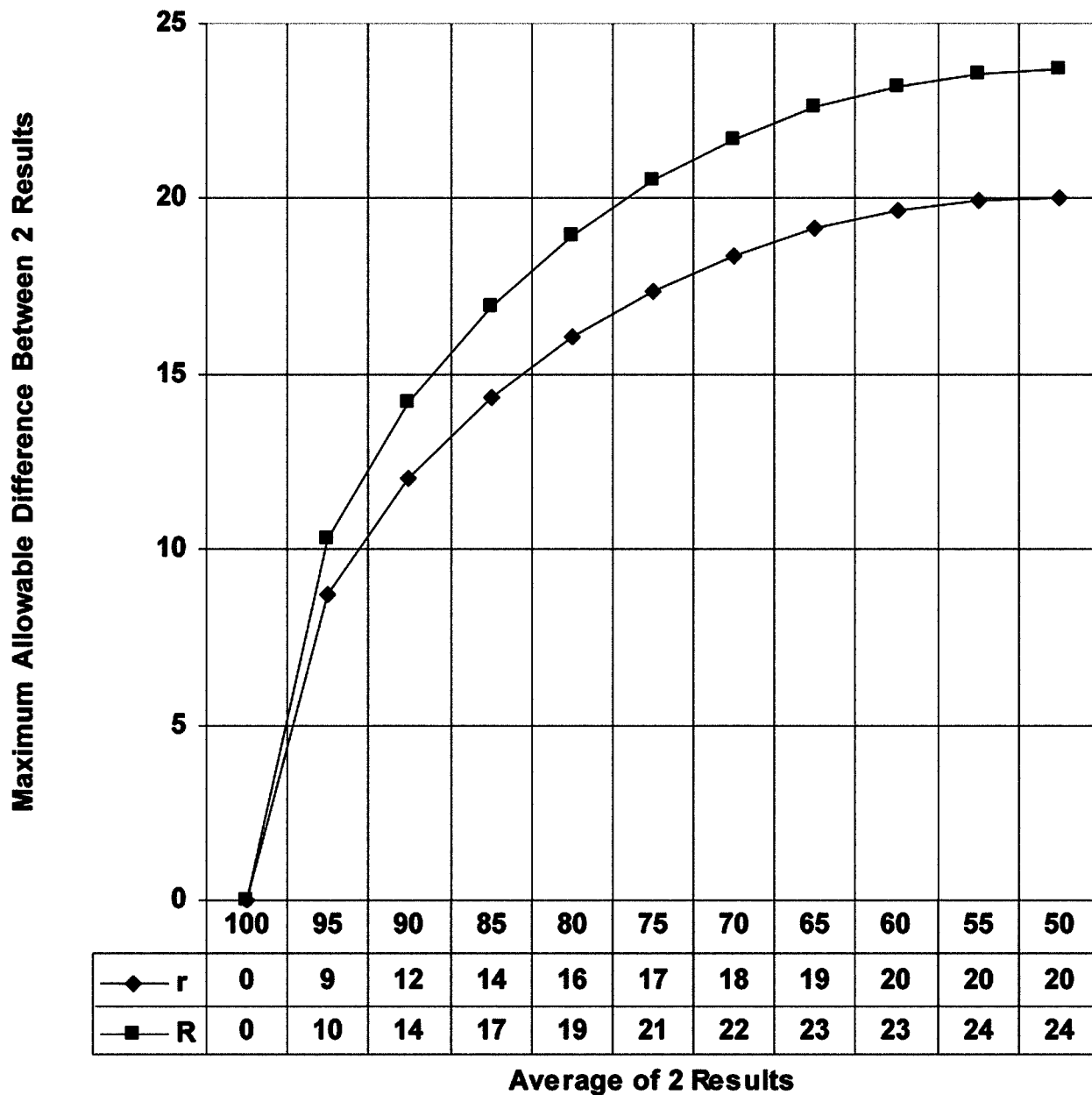
FIG. 14 Field Samples—Variation of Repeatability and Reproducibility of MSEP Ratings Obtained for Field Samples (Jet A, Jet A-1, JP-5, JP-7, and JP-8)
