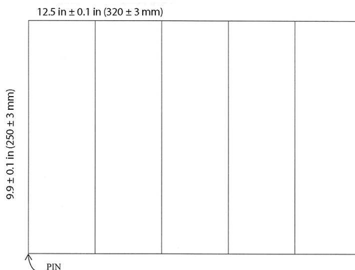
FIG. A2.1 Template for 9.9 by 12.5 in. Specimen
