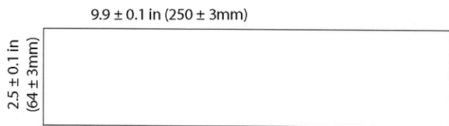
FIG. A2.2 Template for 2.5 by 9.9 in. Specimen
