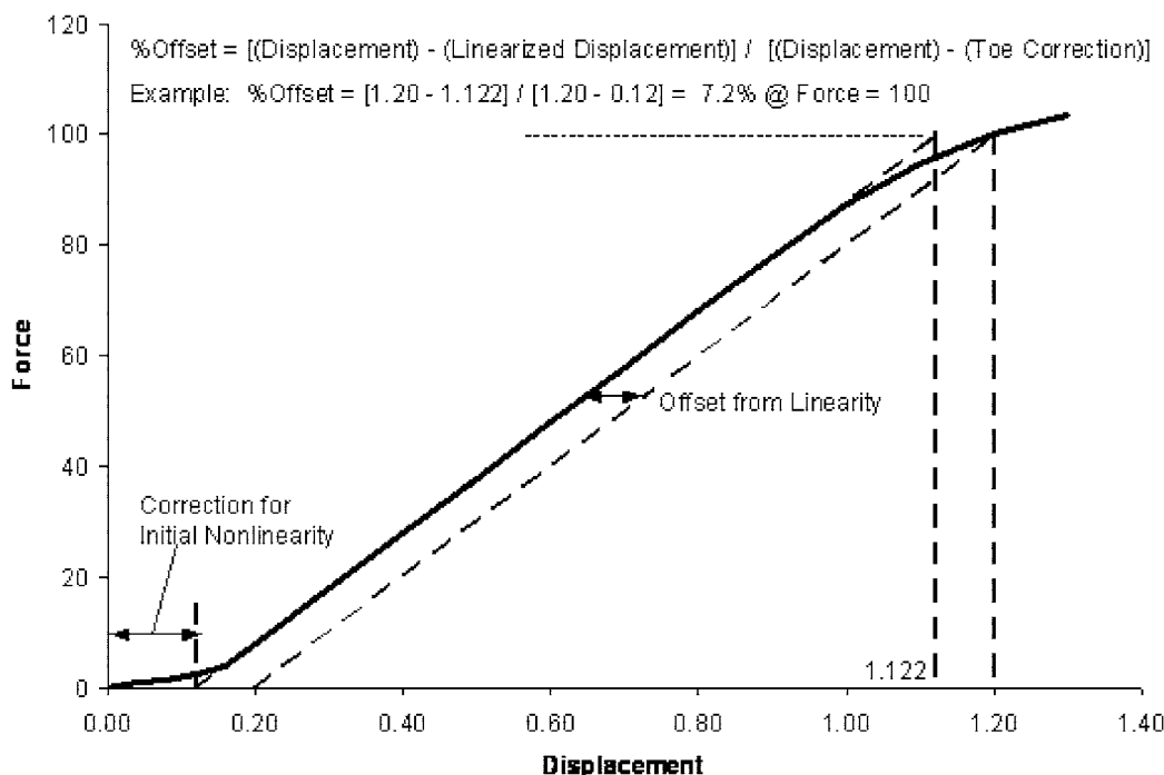
FIG. 2 Determination of Non-Linearity Offset
