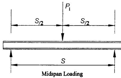
(a) 3-Point Loading (C393/C393M Standard Configuration)
