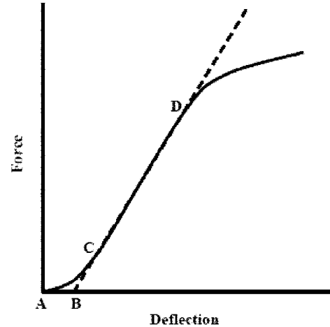
FIG. A1.1 Sandwich Material with Hookean Response Region
