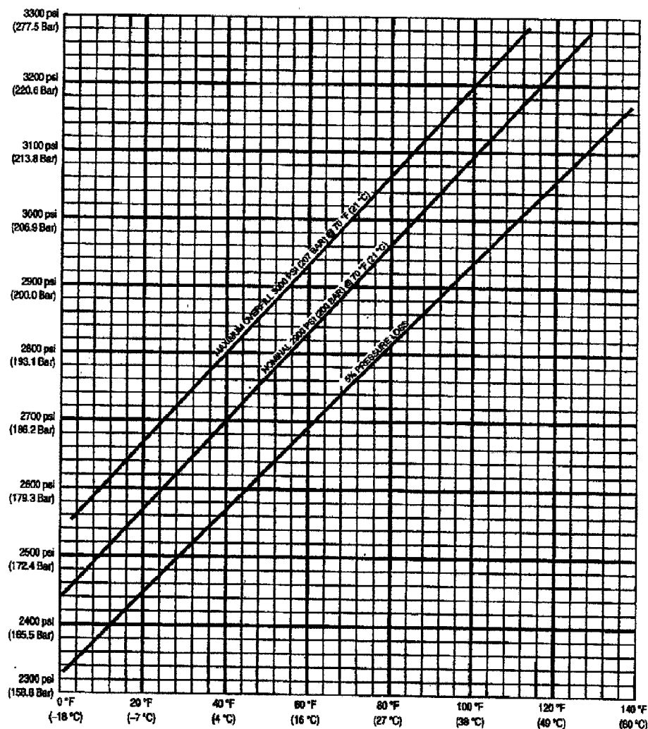
FIG. 2 IG-541 (200 Bar) Isometric Diagram
