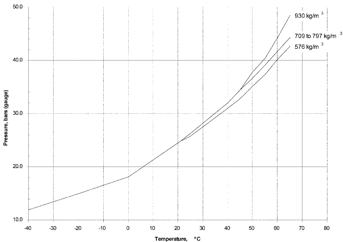
FIG. 5 Isometric Diagram of HFC Blend B Pressurized with Nitrogen to 25 bar @ 21°C—SI Units
