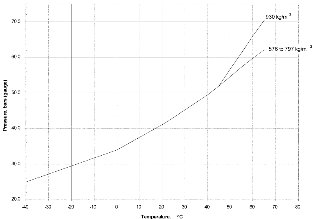
FIG. 6 Isometric Diagram of HFC Blend B Pressurized with Nitrogen to 42 bar @21°C—SI Units
