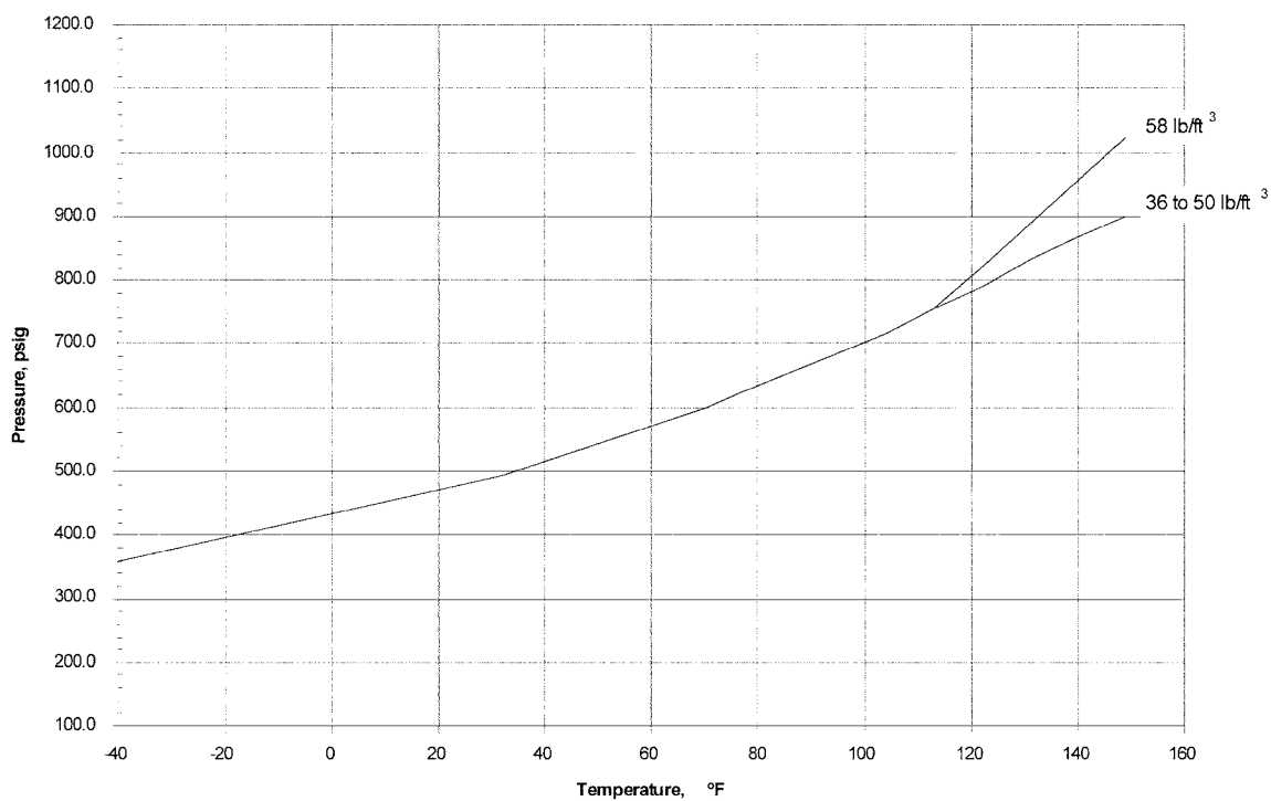
FIG. 4 Isometric Diagram of HFC Blend B Pressurized with Nitrogen to 600 psig @ 70°F—English Units
