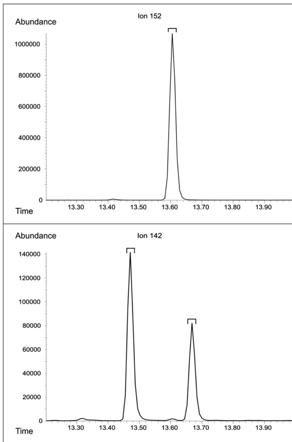
FIG. X1.2 Methylnaphthalenes ("s" is a spiked d 10 -methylnaphthalene surrogate)
