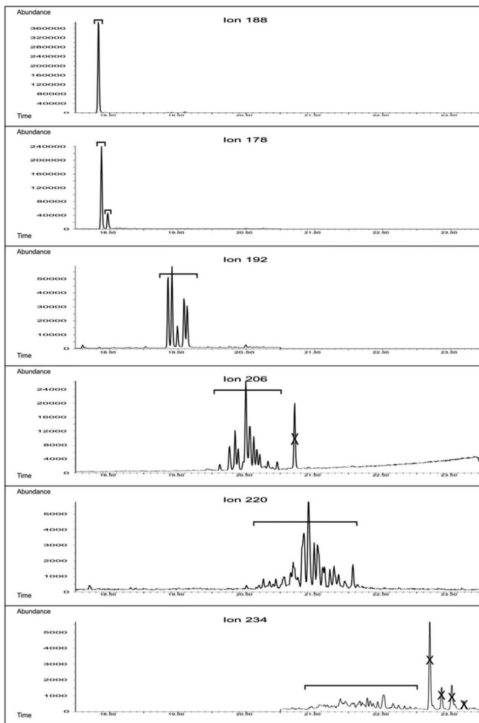
FIG. X1.5 Phenanthrenes/Anthracenes
