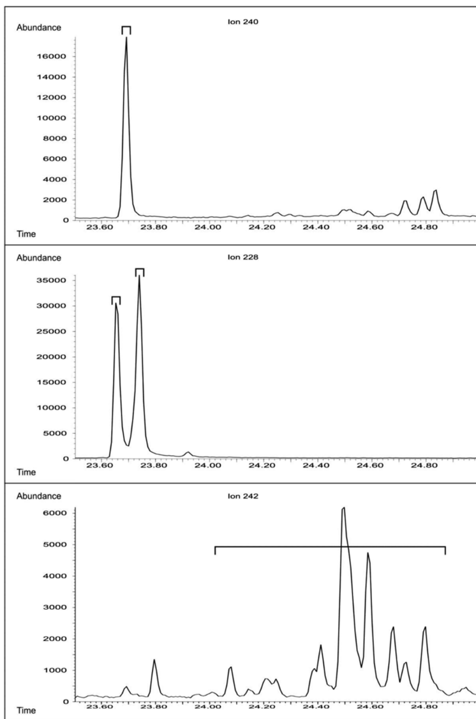
FIG. X1.7 Benz[a]anthracenes/Chrysenes ("s" is a spiked d_{12} -benz[a]anthracene surrogate)
