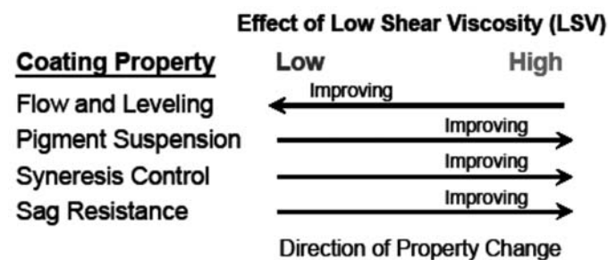
FIG. 1 Low Shear Viscosity (LSV)
