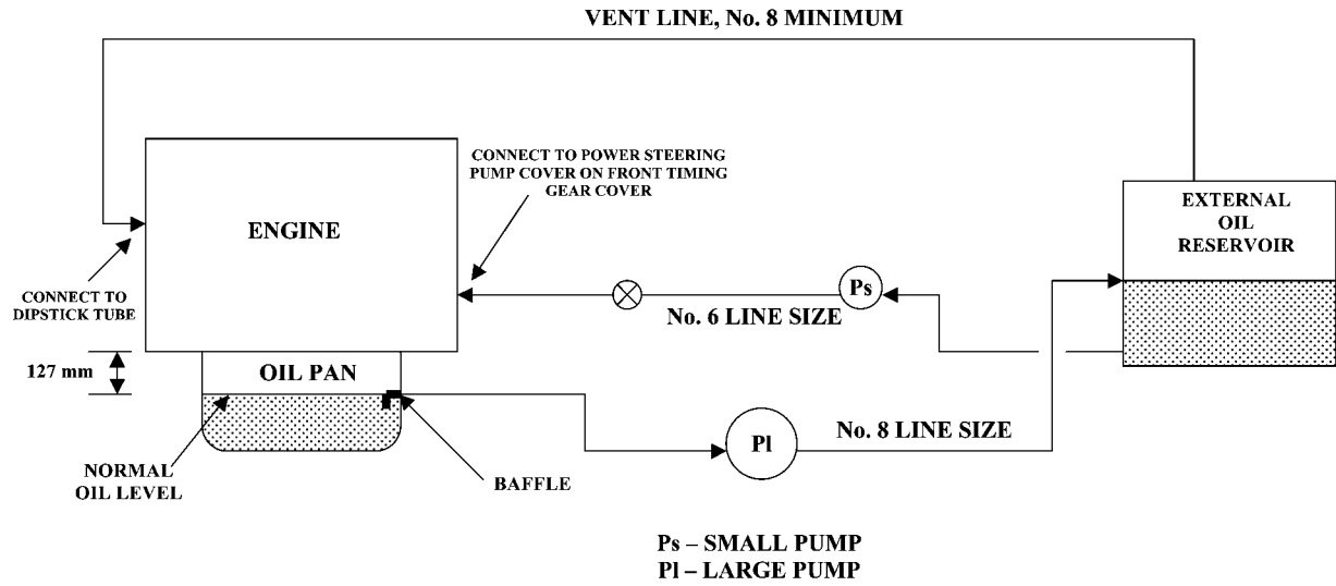
FIG. A1.1 Auxiliary Oil System
