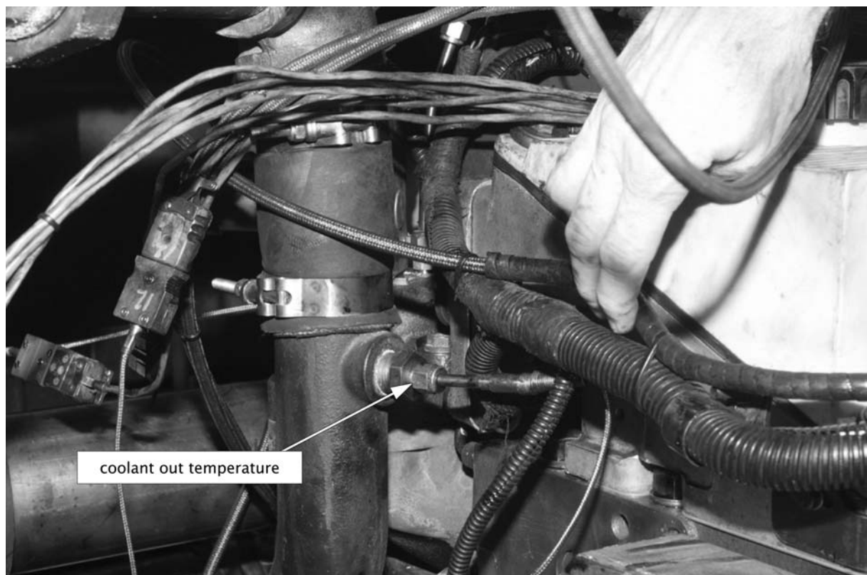
FIG. A4.10 Coolant Out Temperature Measurement Location
