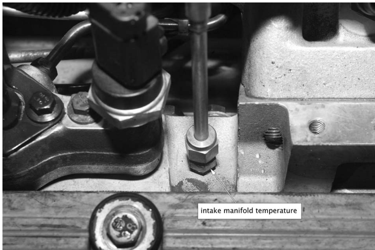
FIG. A4.9 Intake Manifold Temperature Measurement Location Close-up
