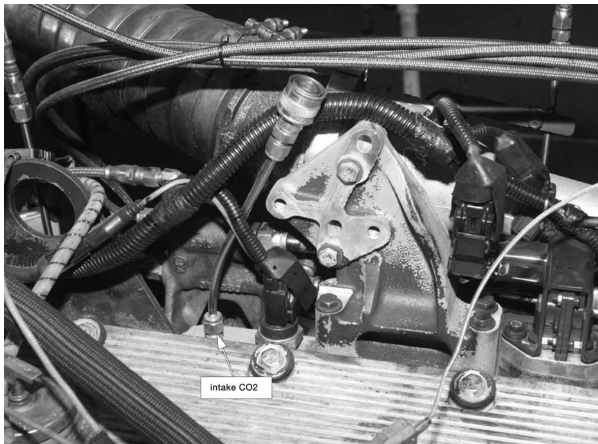
FIG. A4.14 Intake Manifold CO 2 Probe Location
