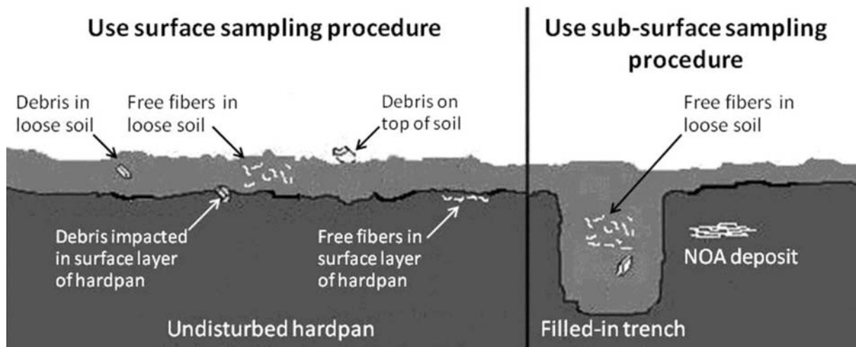
FIG. X2.1 Section through Loose Soil, Hardpan, and Trench (Adapted from Manual on Asbestos Control: Surveys, Removal and Management 8 )
