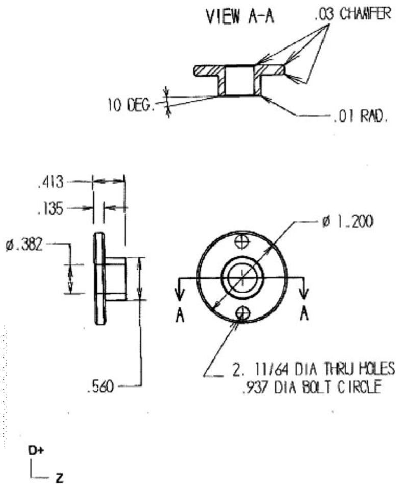
FIG. A5.1 Agitator Packing Gland (all dimensions are in inches) (continued)
