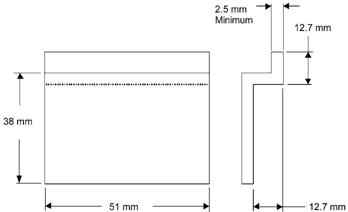
FIG. A4.1 Oil Pan Modifications for External Oil System—Auxiliary Oil System Suction Port Location
