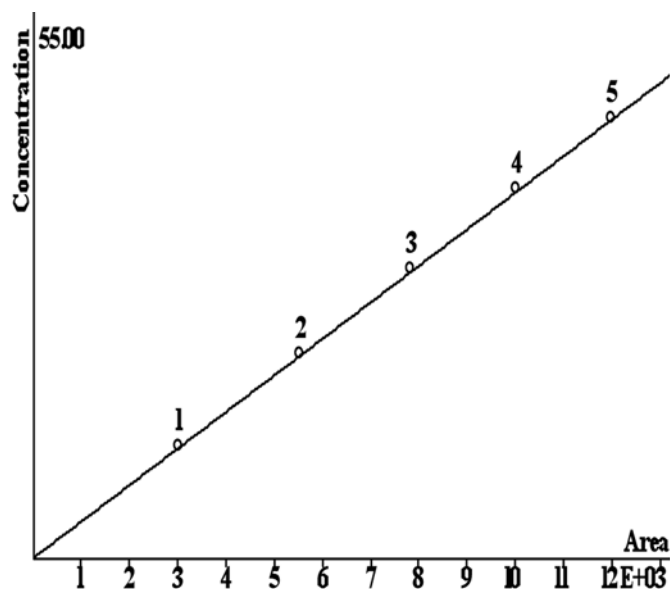
FIG. 2 Typical Glycerin Calibration Plot
