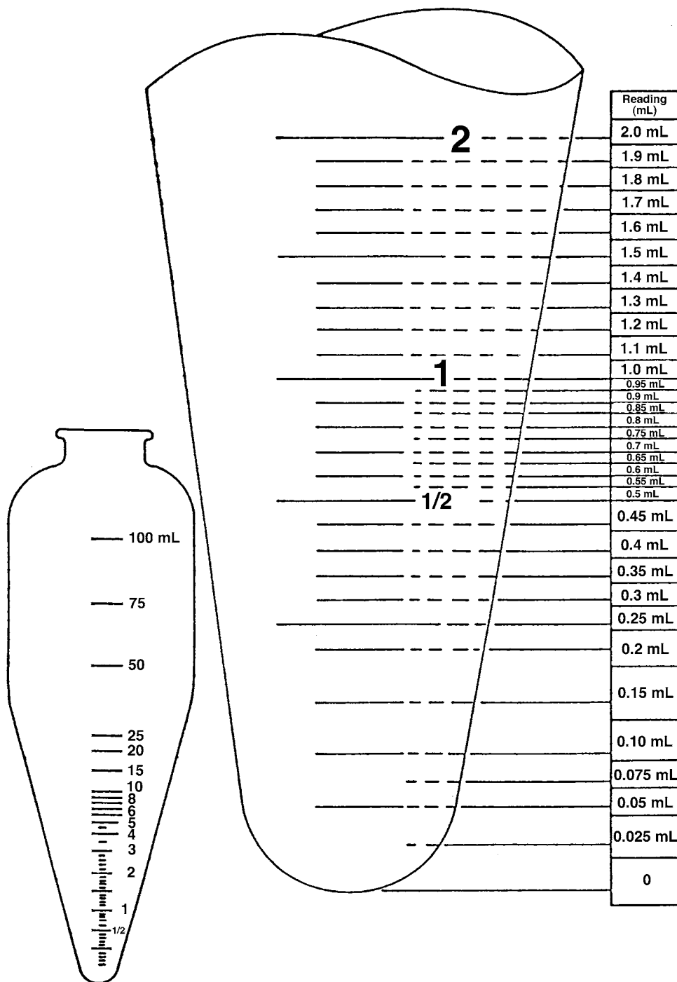
FIG. X1.1 Procedure for Reading Volume of Separated Liquid for the Centrifuge Tube
