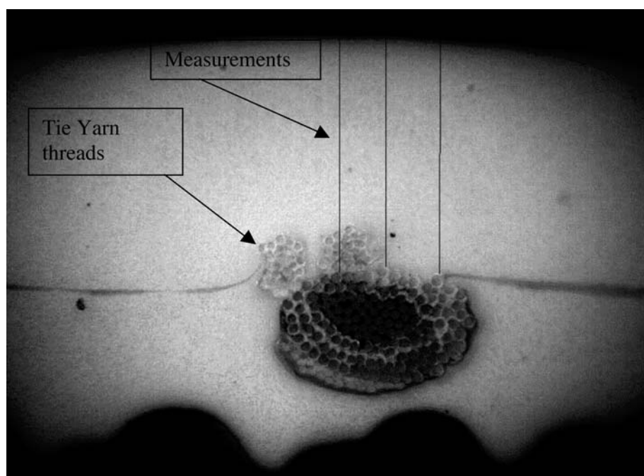
FIG. 3 Representative Area Over Machine Direction Thread
