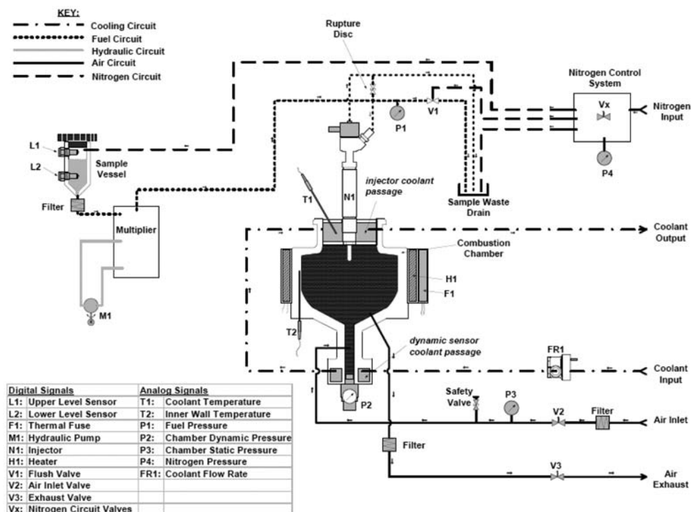
FIG. A4.1 Instrument Schematic
