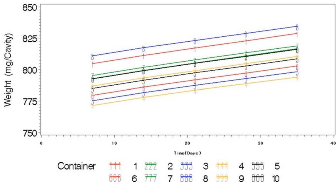
FIG. X1.1 Blister Weights versus Time
