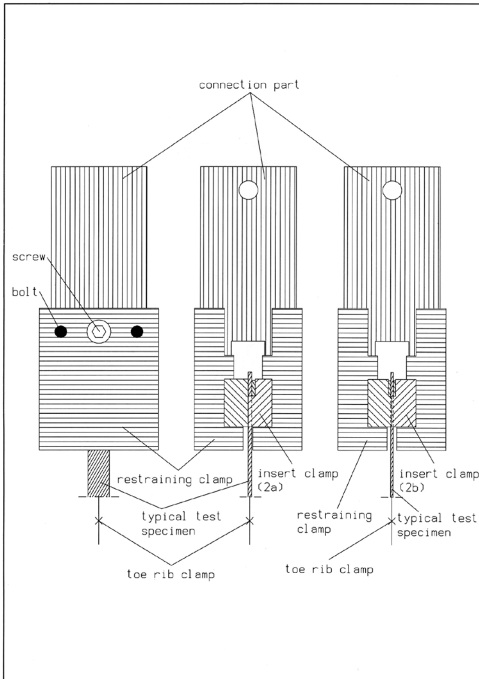
FIG. 4 Entire Assembly for Constrained Rotation of the Geogrid Junction per Section 6.4
