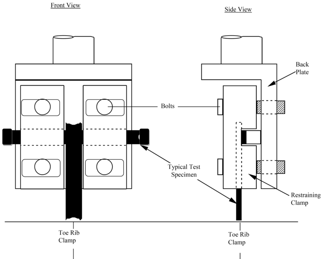
FIG. 1 Typical Junction Strength Test Specimen Test Setup [Rotation is not Constrained per Section 6.3]
