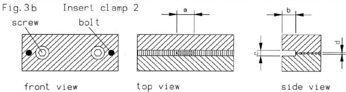
FIG. 3 Alternative Clamp for Constraining Rotation of the Geogrid Junction per Section 6.4
