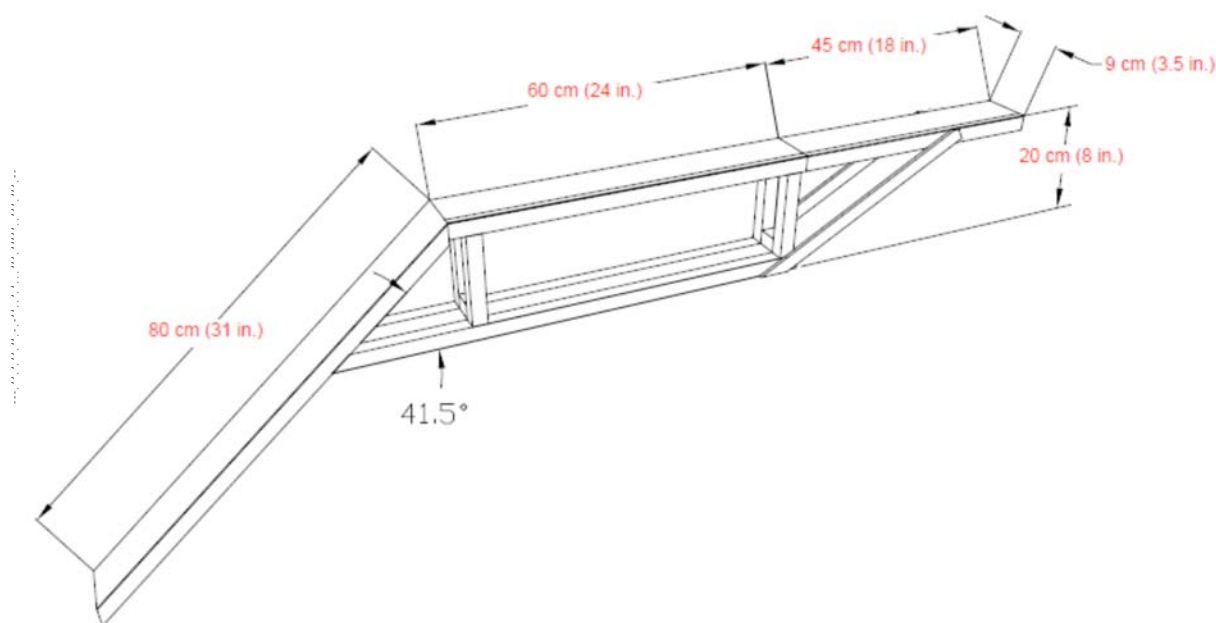
FIG. 1 Example Test Rig Setup
