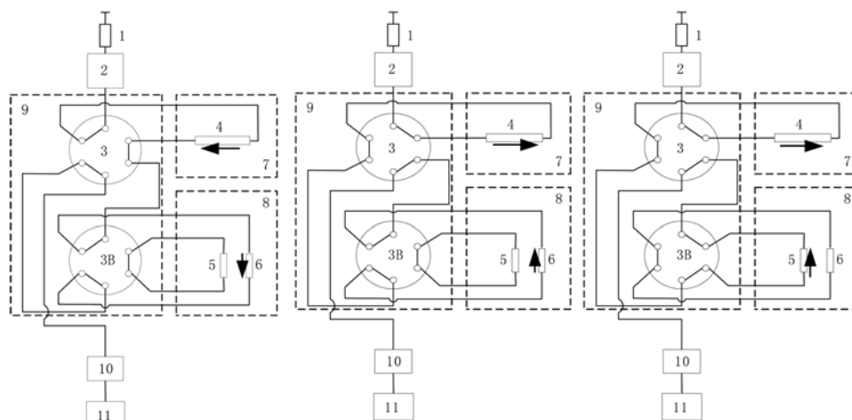
FIG. 6 Valves Positions During Analysis
