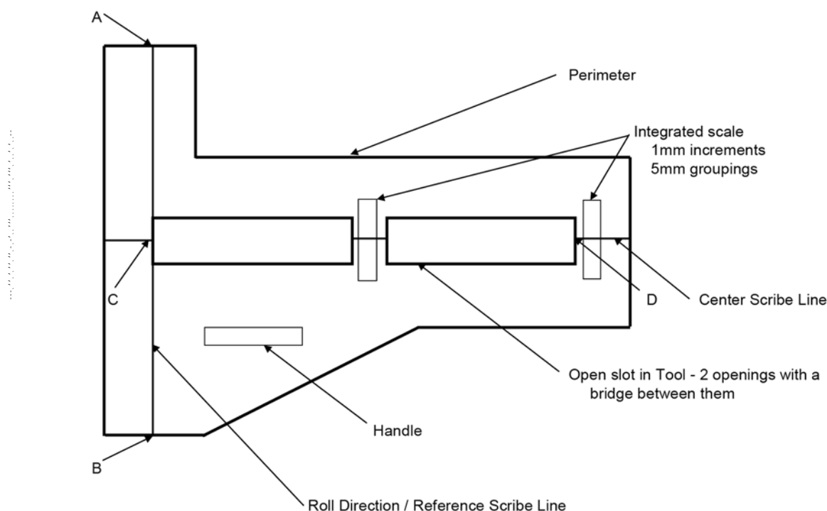
FIG. 1 Bow Skew Tool with Open Slot
