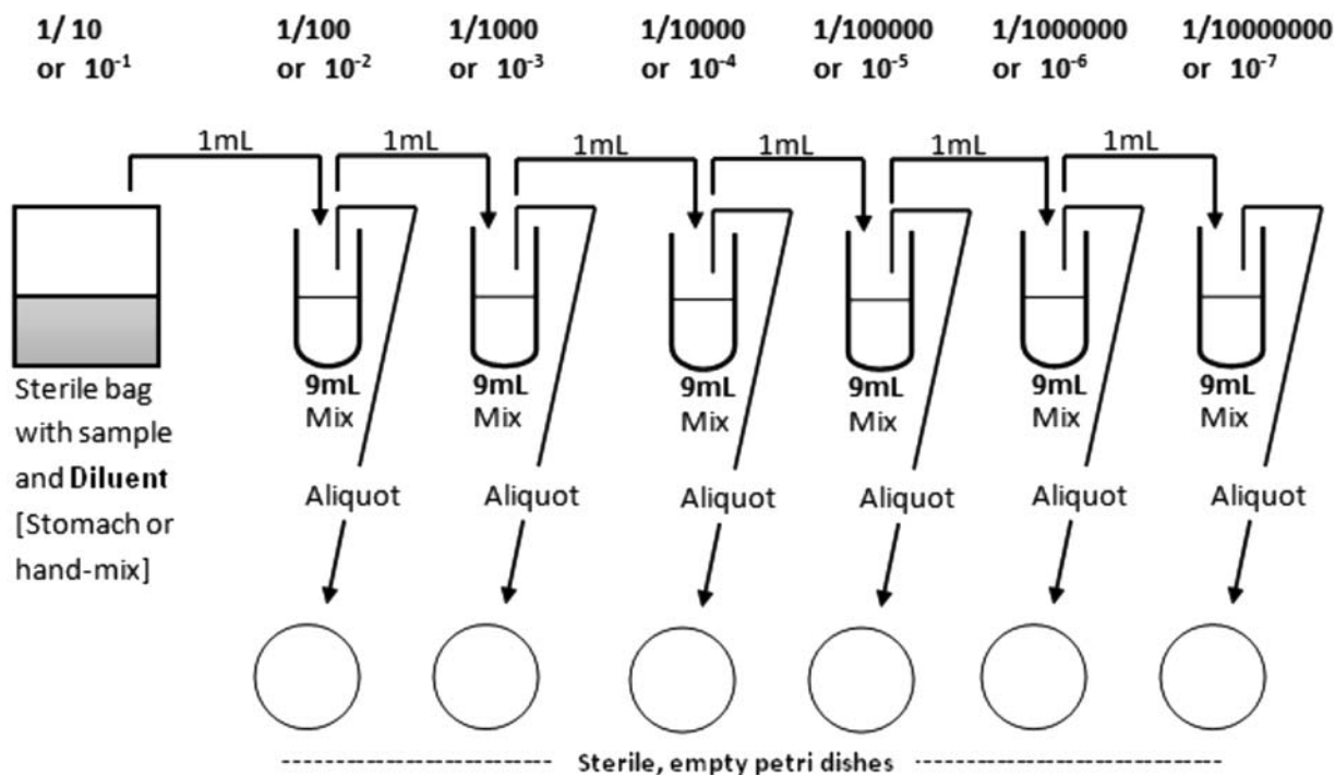
FIG. 1 Plating
