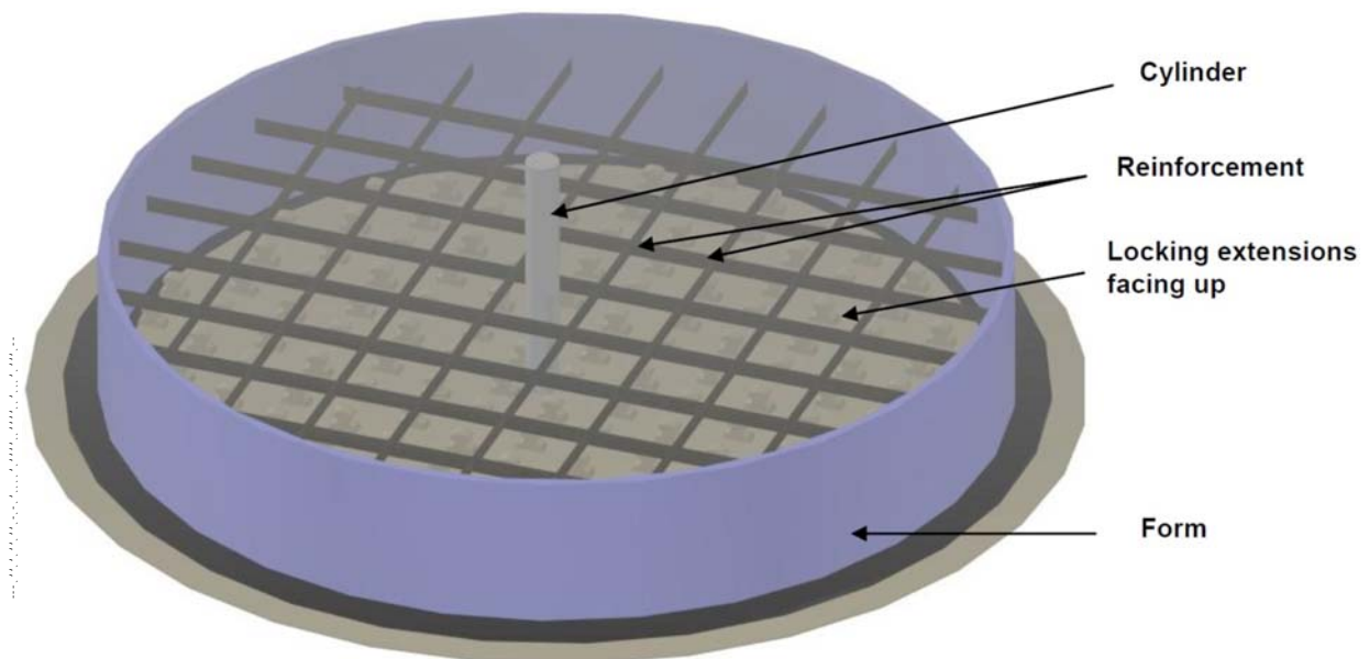
FIG. 2 Bottom of Form with Studs facing up and cylinder spacer
