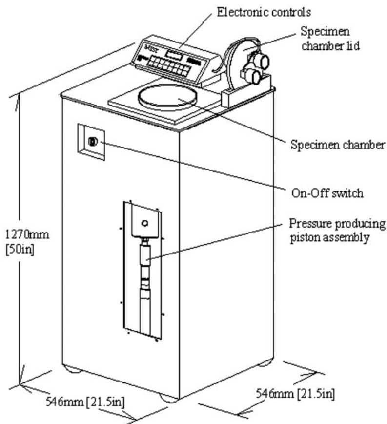
FIG. 1 Moisture Conditioning System
