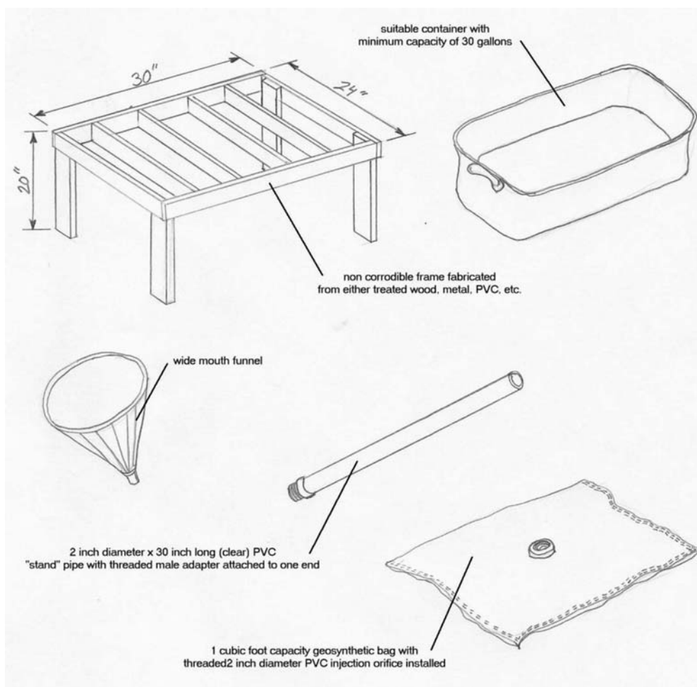
FIG. 1 Test Equipment, Bag and Frame
