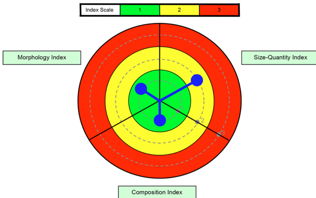
FIG. X2.2 FDA Triplex Plot Indicated Moderate Number and/or Size of Particles with Composition and Morphology Consistent with Benign Debris—No Further Action Required
