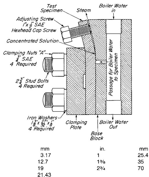
FIG. 1 Cross-Section of Embrittlement Detector
