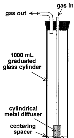
FIG. X2.2 Set-up of Graduated Cylinder with Spacer
