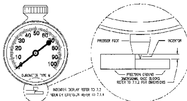
FIG. 4 Detail of Indentor Extension &amp; Display Adjustment
