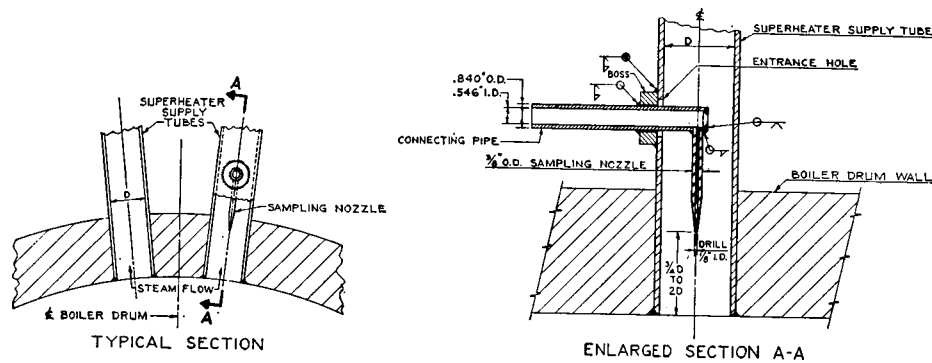
FIG. 3 Steam Sampling Nozzle, Single-Port Type
