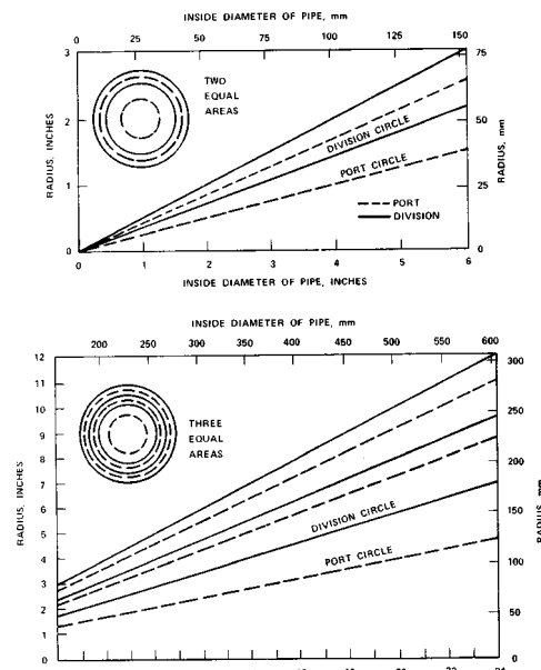
FIG. 6 Radii of Circles for Dividing a Circular Pipe into Annuli of Equal Areas
