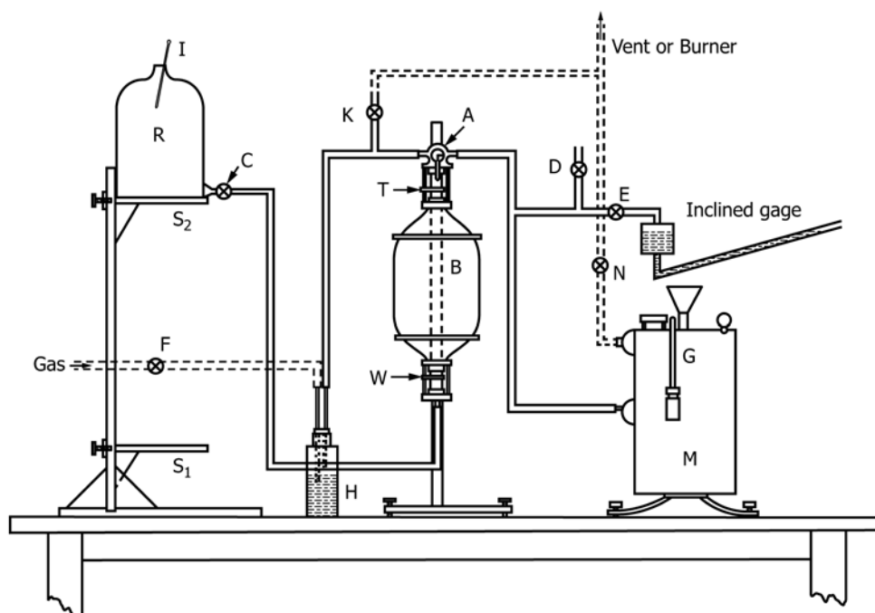
FIG. 5 Schematic Diagram of Equipment and Connections for Calibration of a 0.1-ft 3 Wet Test Meter with a 0.1-ft 3 Bottle
