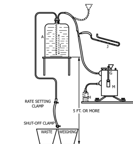
FIG. 6 Simple Equipment for Calibration by Aspirator Method
