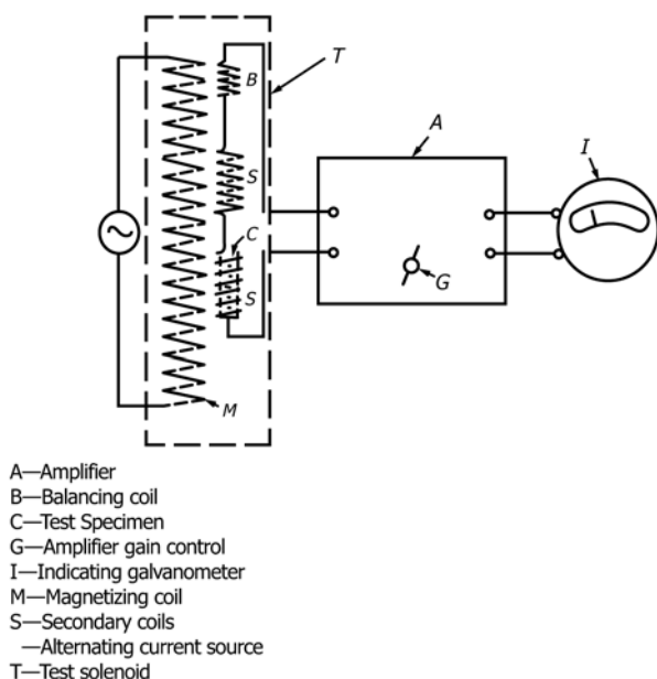
FIG. A1.1 Schematic Diagram of the Mapes Analyzer
