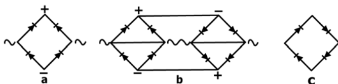
FIG. A2.6 Schematic Diagram of Rectifiers and Connections
