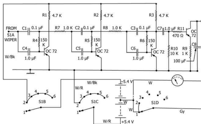
FIG. A2.4 Magnetic Analyzer—Amplifier, Meter, and Switching
