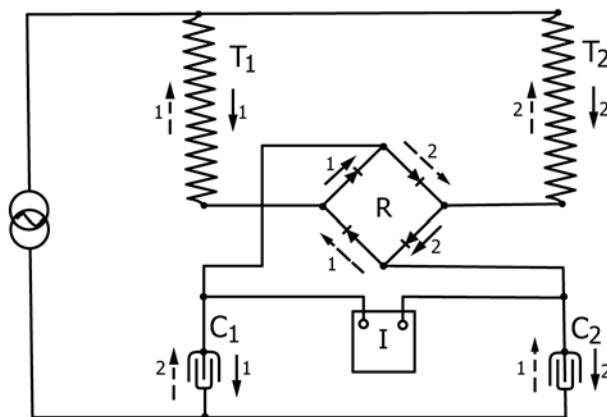
FIG. A2.5 Schematic Diagram of Apparatus
