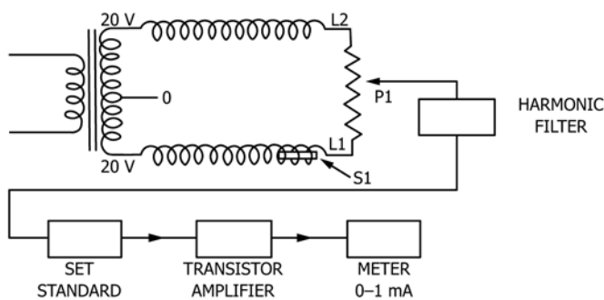
FIG. A2.2 Magnetic Analyzer—Principle of Method
