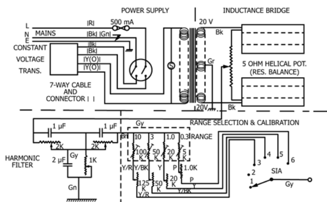
FIG. A2.3 Magnetic Analyzer—Power Supply, Bridge, Harmonic Filter, and Range Selector
