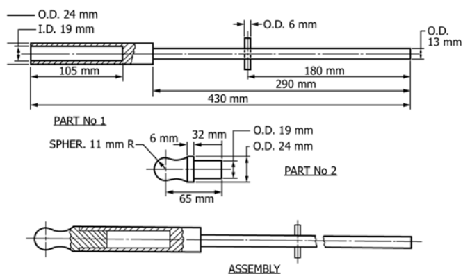
FIG. A1.2 Specimen Holder
