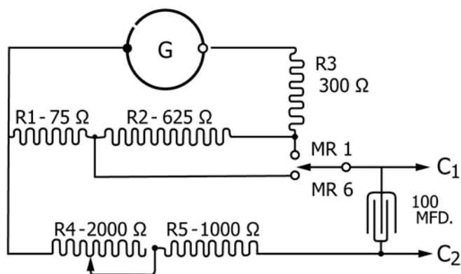
FIG. A2.7 Schematic Diagram of Indicating Instrument
