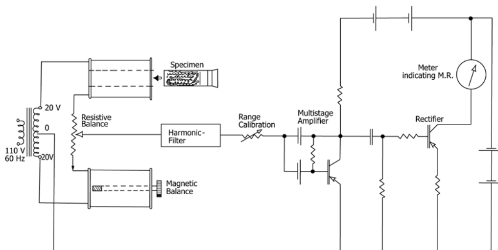
FIG. A2.1 Schematic Diagram of Turner & Newall 5 Magnetic Analyzer
