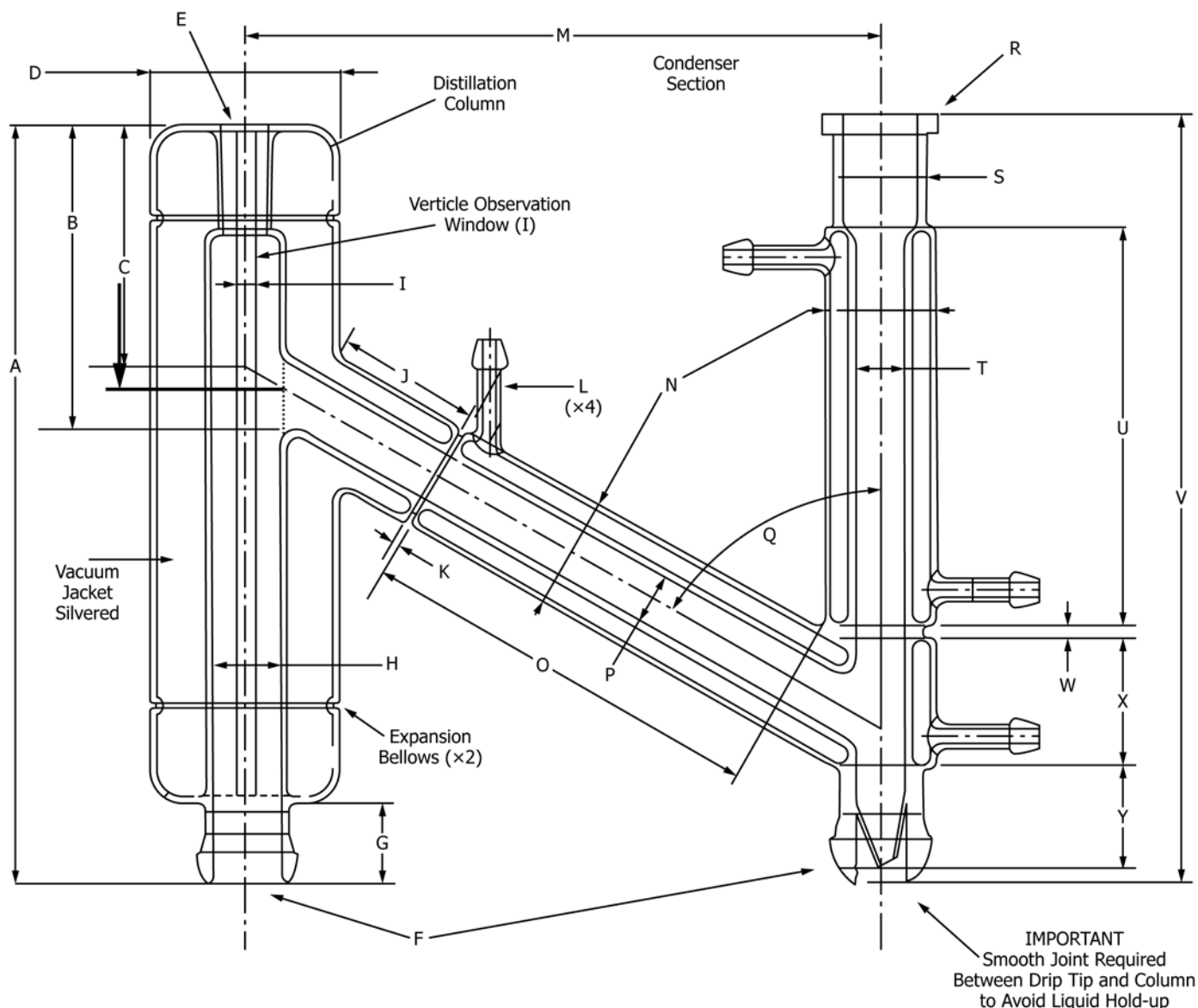
FIG. 4 Vacuum-Jacketed Column
