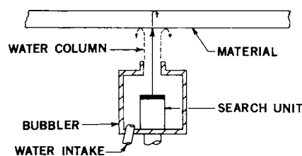
FIG. X2.1 Bubbler Setup
