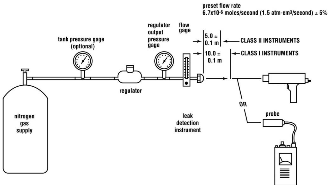
FIG. 1 Calibrated Leak Standard/Sensitivity Validation Equipment
