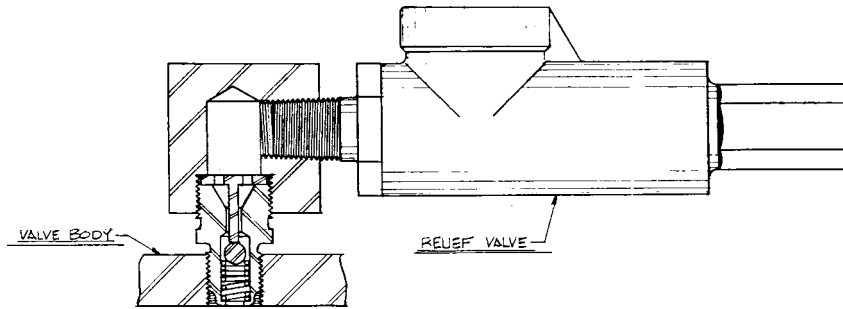
FIG. 1 Assembled Valve-body Pressure-relief Device
