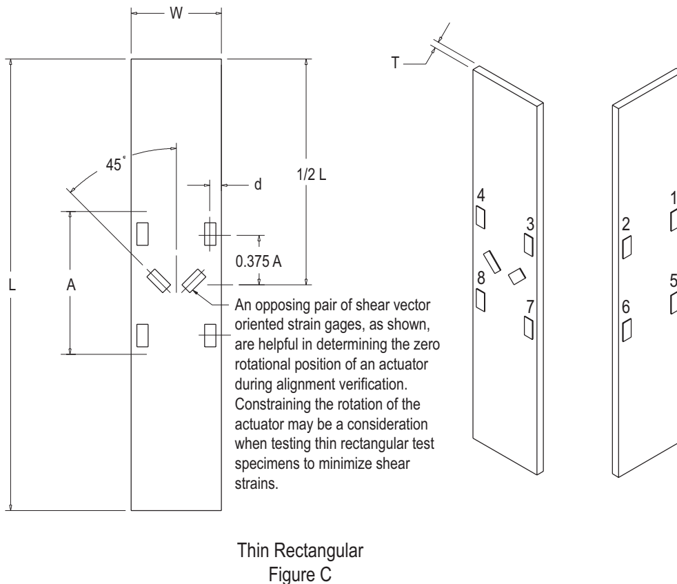
FIG. 3 C Locations of Strain Sensors on (A) Cylindrical, (B) Thick rectangular and (C) Thin Rectangular Strain-Gaged Alignment transducers (Numbers Indicate Positions of Strain Sensors) (continued)
