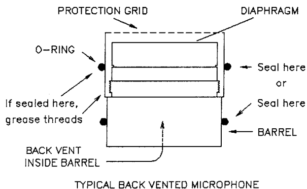
FIG. 2 Microphone Venting and Sealing
