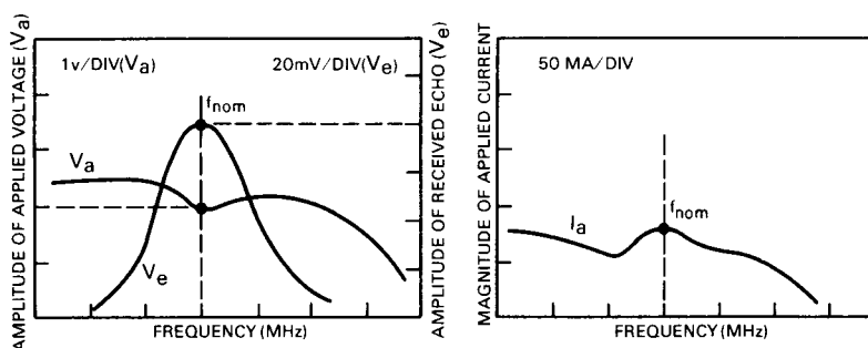
FIG. A5.1 Typical Voltage and Current Recordings for Determining Magnitude of Search Unit Impedance
