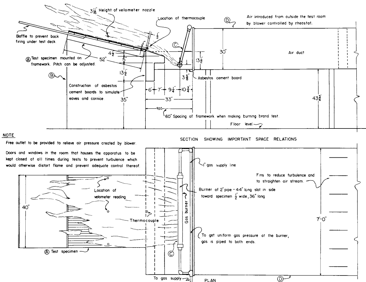
FIG. 1 Schematic Drawing of Fire Test Apparatus
