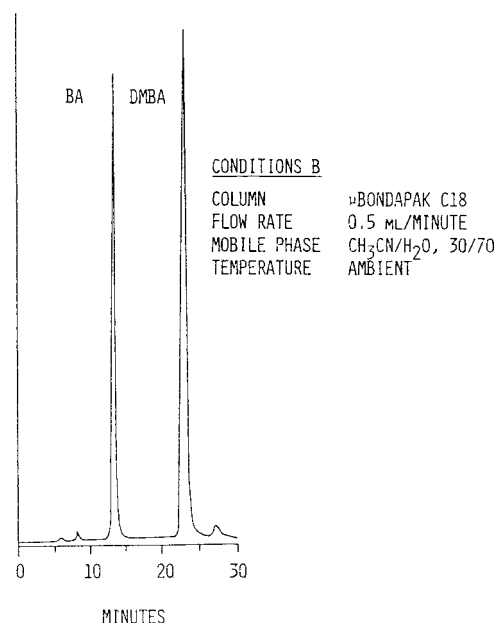
FIG. 4 Typical Chromatogram for Dimethylbenzyl Alcohol Calibration
